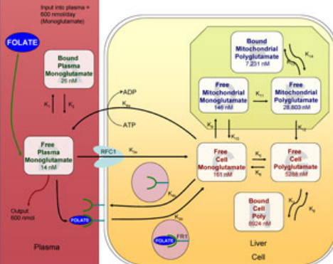
Figure 2. Transport pool concentrations of folate in the plasma and in the liver cell. K in represent rates of transport, transport and binding.
